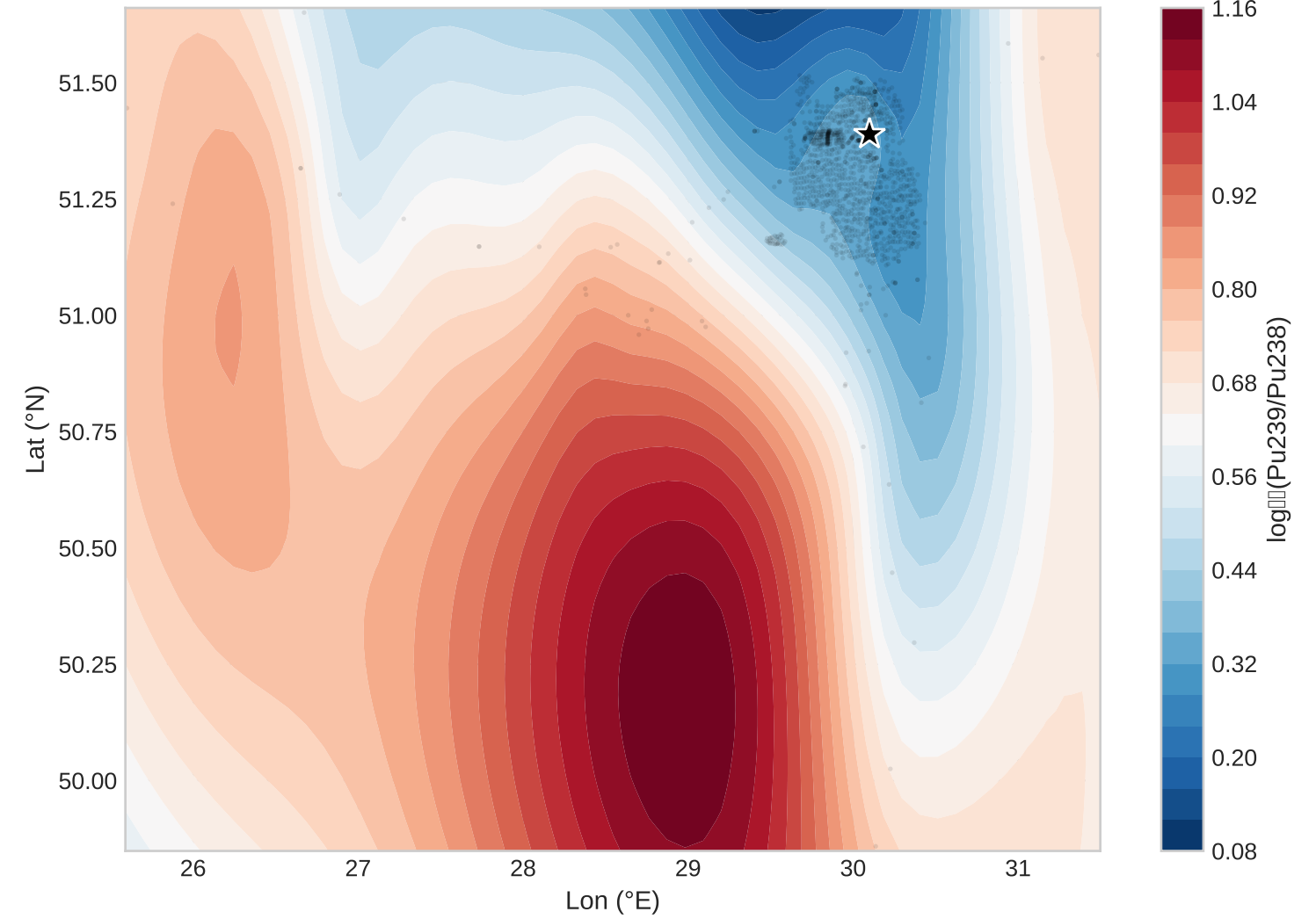
Pu239/Pu238 (Burnup indicator) \mu=0.71 \pm 0.22
